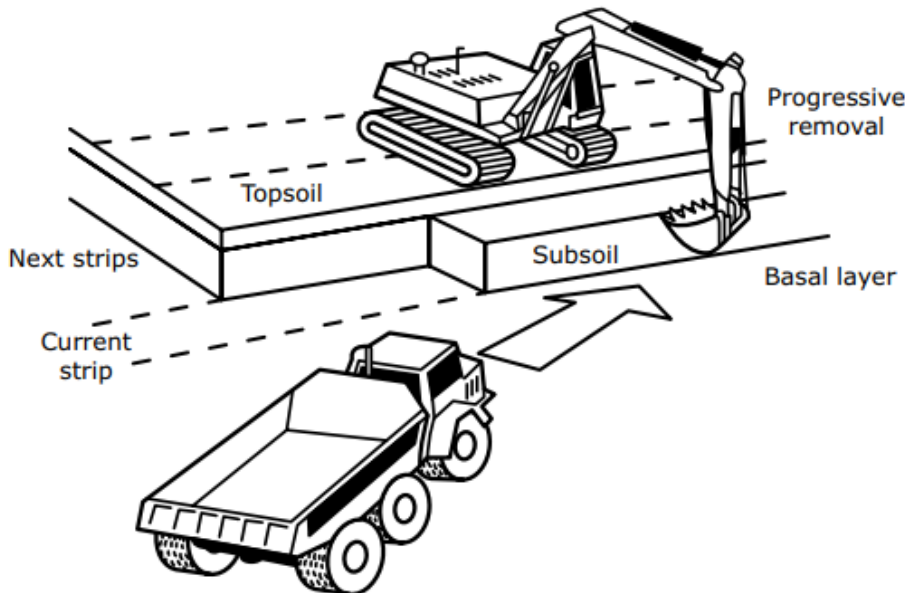
Plate 2: Stripping with excavators and dump trucks: removal of subsoil from a strip. Reproduced from Part 2: Sheet A of IoQ (2021) (Ref. 3).
