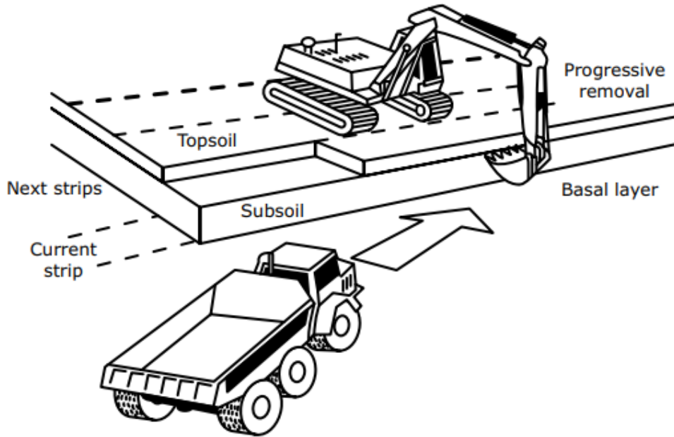
Plate 2: Stripping with excavators and dump trucks: removal of subsoil from a strip. Reproduced from Part 2: Sheet A of IoQ (2021) (Ref. 3).
